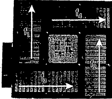
Figure 1: A planar motor with integral sensing: four linear actuators combine to generate forces and a torque in the plane.
