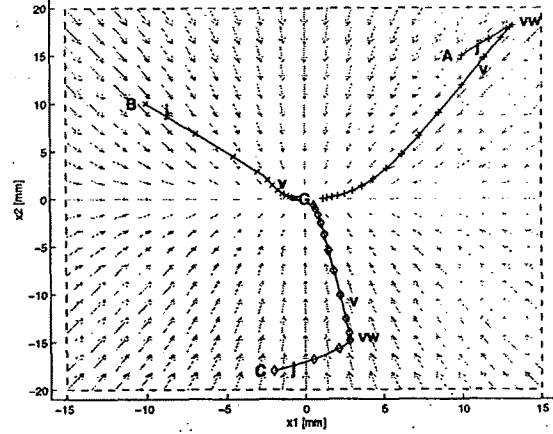
Figure 3: Position traces for three simulations A, B, C with different starting conditions but identical boundary \mathcal{P} (dashed lines). Controller switches are indicated by codes (j=join, vw=velocity controller in \mathcal{N}_w , v=velocity controller in \mathcal{N}_v ). Symbols (+, x, o) demarcate 5 msec time intervals.
