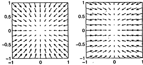
Figure 2: A vector field \hat{v} derived from (9) defines a desired velocity at each position for the controller. (left: \alpha_1 = \alpha_2 = 5 , right: \alpha_1 = 2, \alpha_2 = 8 )
